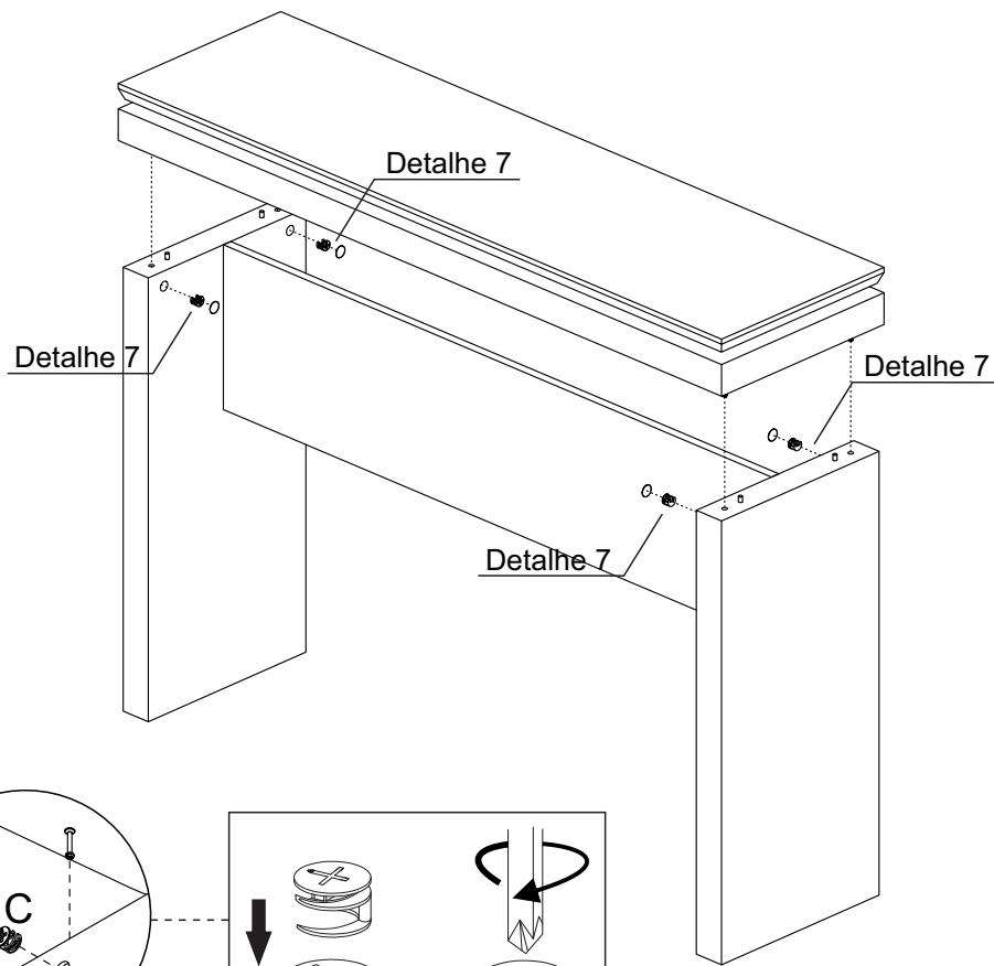
Detalhe 7 Detalle/Detail
