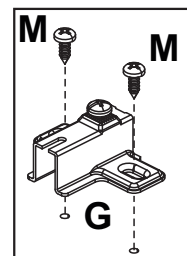
Detalhe 4 Detalle/Detail
