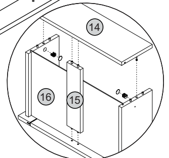
Detalhe 12 Detalle/Detail
