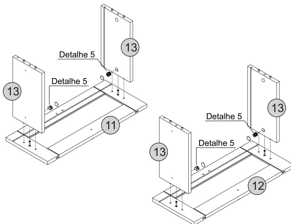
Detalhe 5 Detalle/Detail
