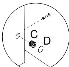
Detalhe 5 Detalle/Detail
